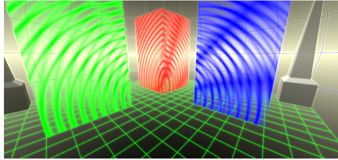
Figure 2: Special volumes sketch
